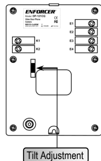
Figure 6 – Rear of Camera Unit
