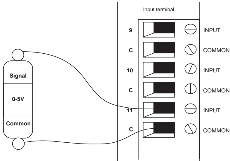
Figure 8: 0-5V sensor
