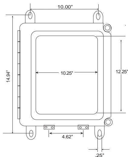
Figure 1: Mounting dimensions
