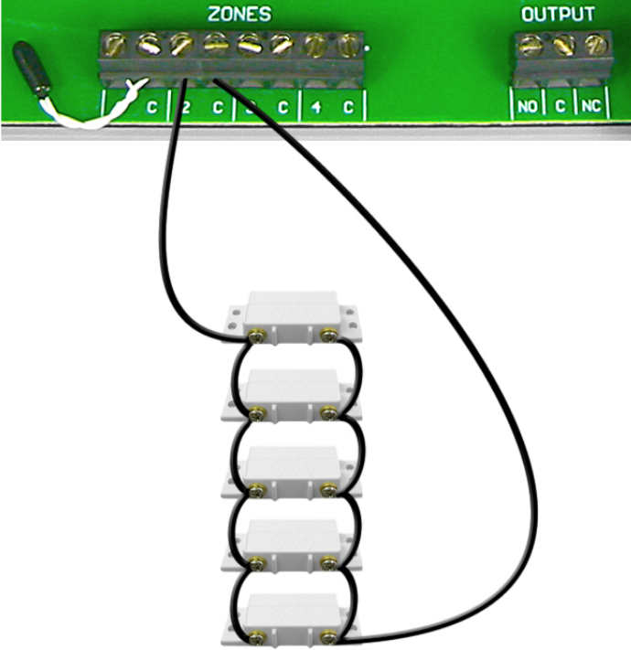
WIRING FOR NORMALLY OPEN (NO) DEVICES IN PARALLEL
