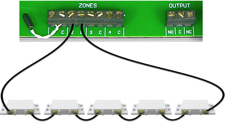
WIRING FOR NORMALLY CLOSED (NC) DEVICES IN SERIES
