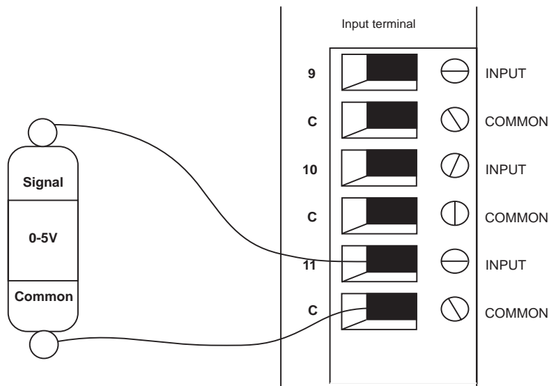
Figure 8: 0-5V sensor
