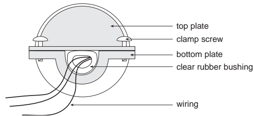
Figure 9: Strain relief clamp
