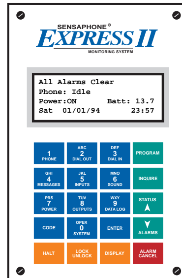
Figure 5-1: Express II Local Display and Keypad
