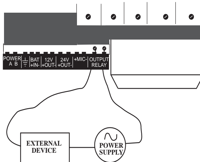
Figure 12: Location of On-board Output relay
