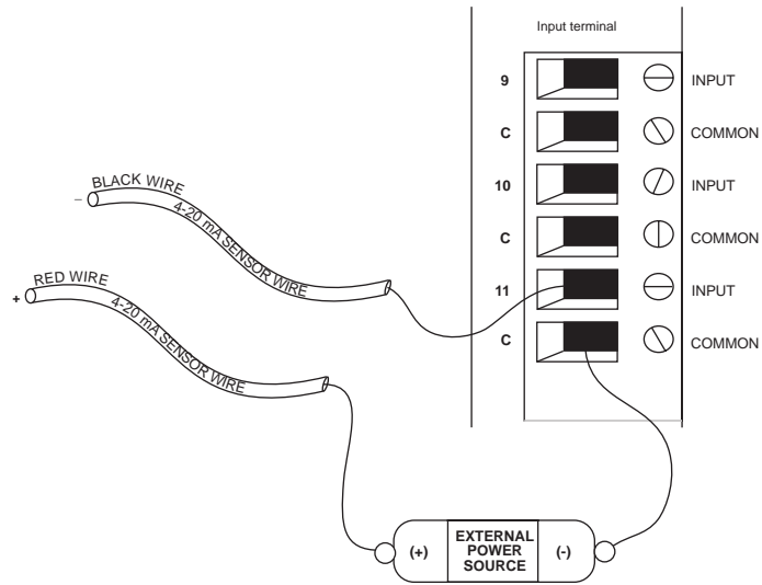
Figure 7: 4-20mA sensor using external power source
