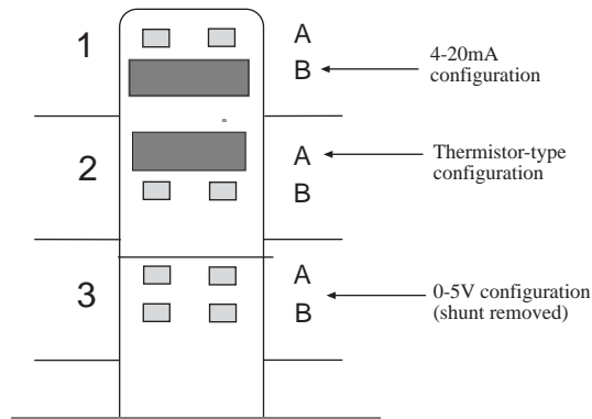
Figure 4: shunt configurations
