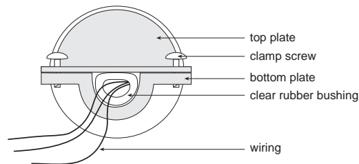
Figure 2: Strain relief clamp
