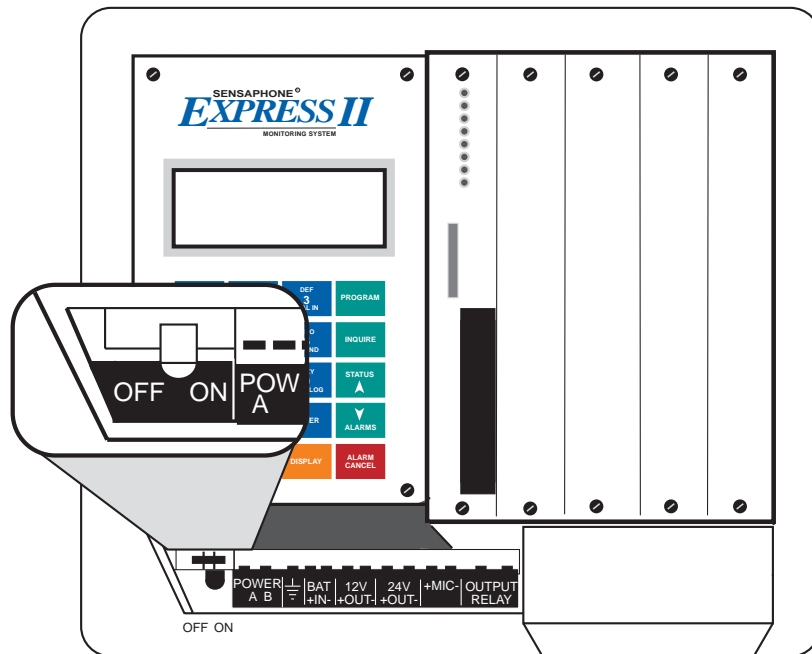
Figure 3: On/Off Switch Location
