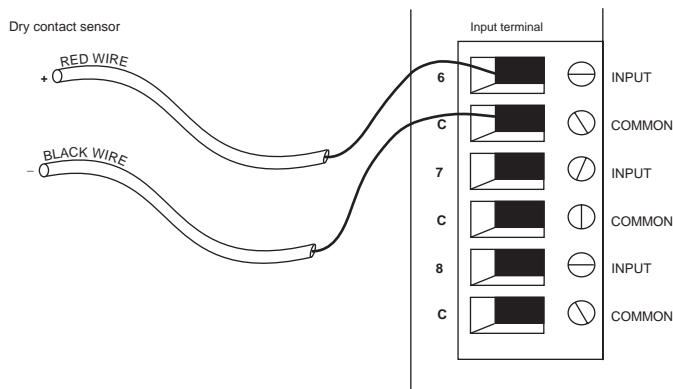
Figure 5: Dry contact sensor
