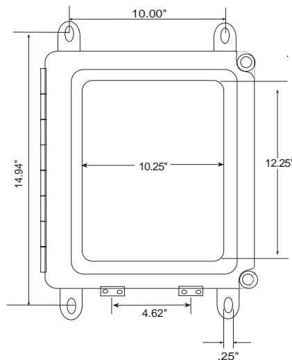
Figure 1: Mounting dimensions
