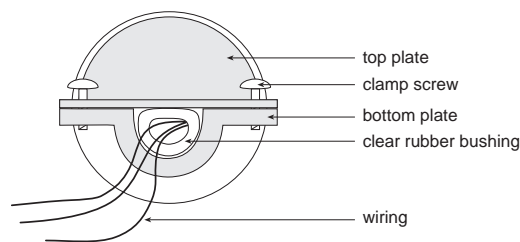
Figure 13: Strain relief clamp
